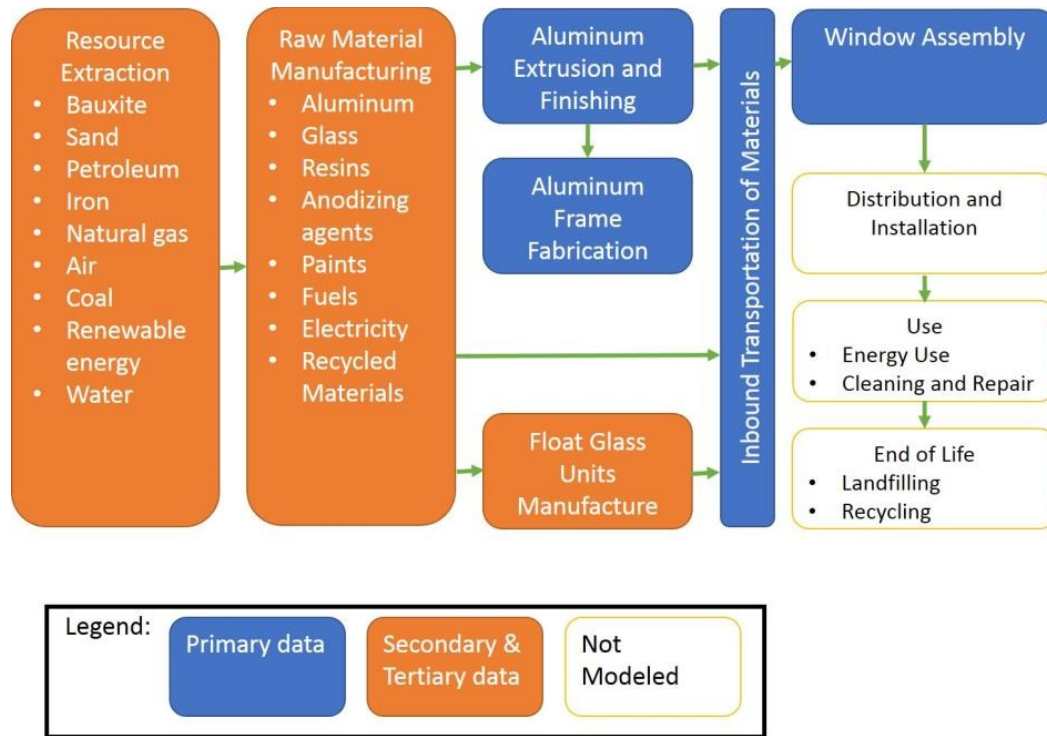
Figure 2. Life cycle stage diagram for cradle-to-gate production of overhead glazing
