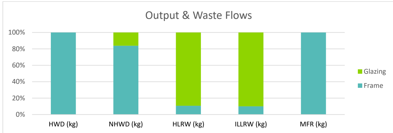
Figure 5. Overhead curtain wall output and waste flows (zero values are not shown in the graph)
