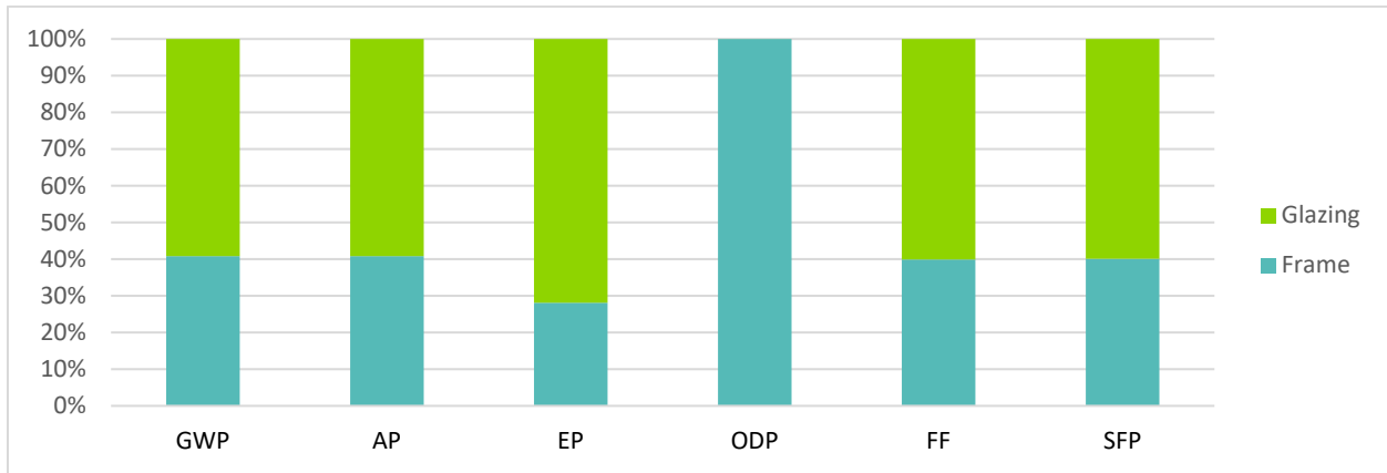
Figure 3. TRACI Impact Categories for overhead curtain wall
