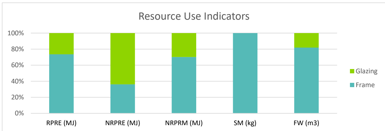
Figure 4. Overhead curtain wall resource use indicators (zero values are not shown in the graph)
